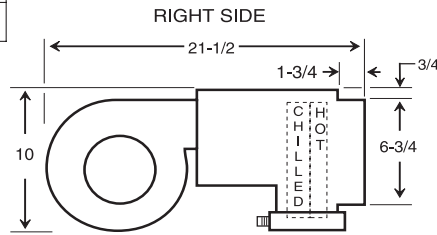
4 - PIPE UNIT SHOWN
