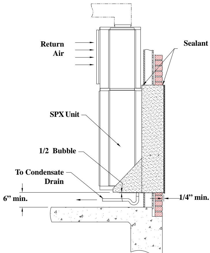
Figure 4 - Side View
